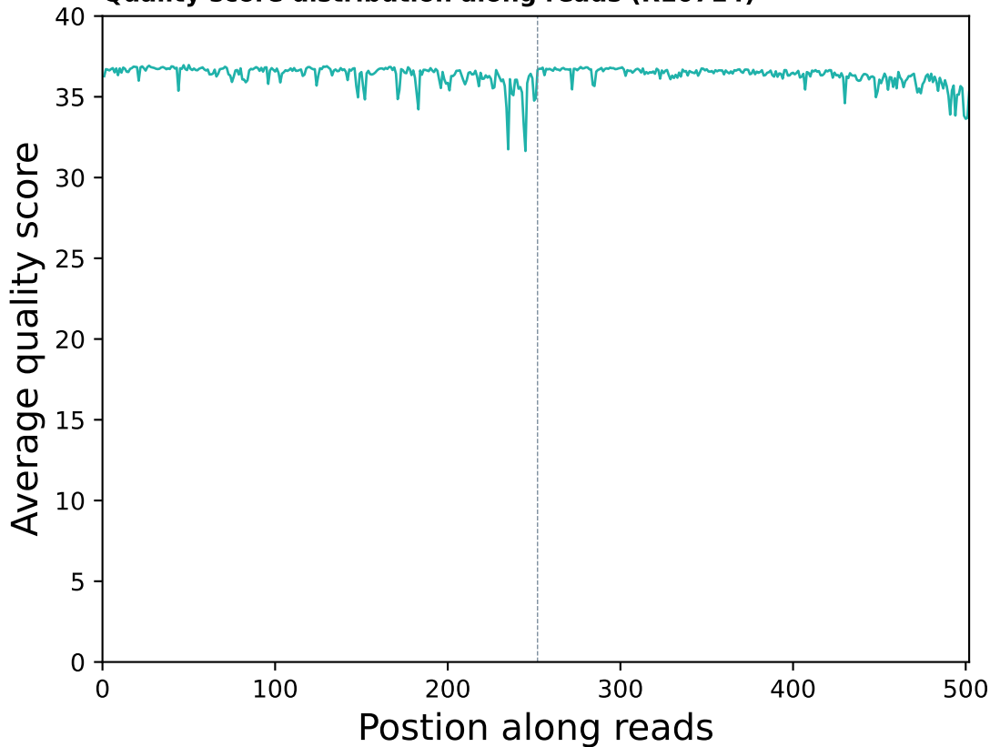
Quality score distribution along reads (R10714)
